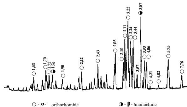
Fig. 2. X-ray of sulfur
